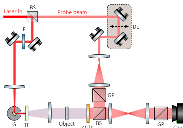
Fig. 28 | Schematic diagram illustrating the single-scan terahertz field spatio-temporal detection 216 .
