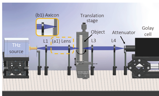
Fig. 14 | Device diagram of the terahertz CT system based on Bessel beams. Figure reproduced with permission from ref. 33 , Optica Publishing Group.
