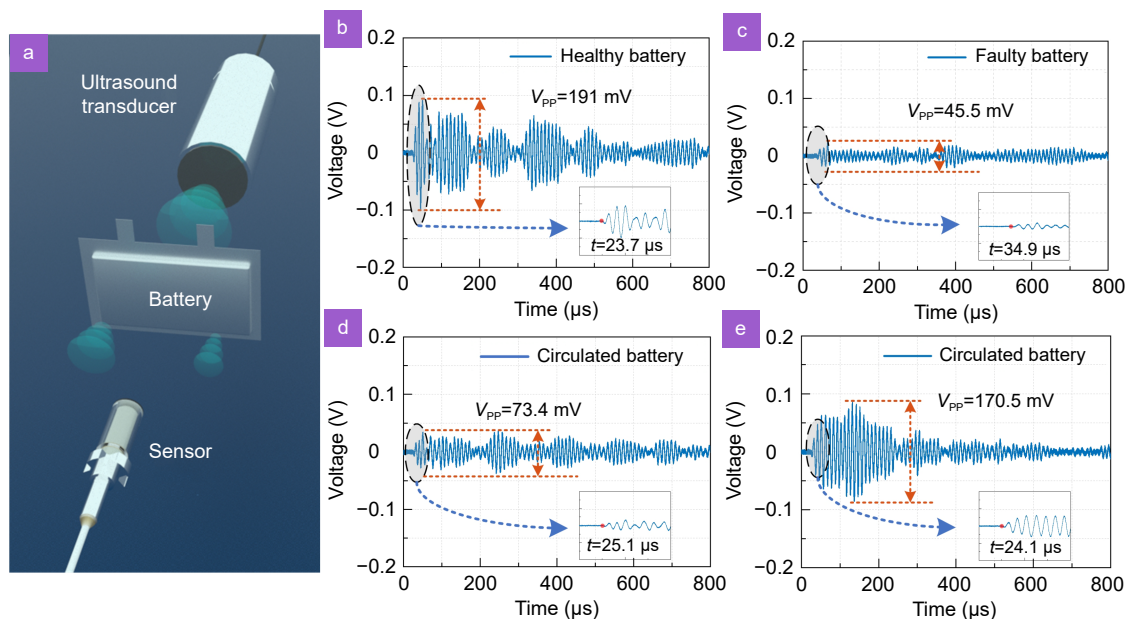
Fig. 3 | (a) The simplified experiment setup of the fixed-point detection. Signals from the LFP||Gr batteries which are (b) healthy and (c) faulty. (d, e) Signals from different parts of the battery which cycles for 2000 times, respectively.
