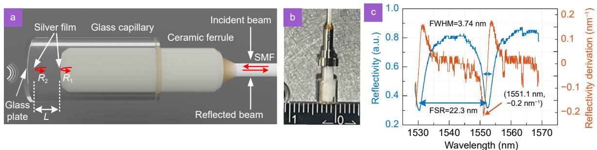
Fig. 1 | (a) Schematic of the fiber optic FPI ultrasound sensor tip. (b) Photograph of the sensor tip. (c) The reflected spectrum and its derivation of the fiber optic FP ultrasound sensor.
