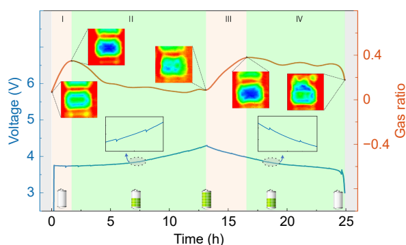
Fig. 6 | The galvanostatic curves and gas ratio variation of the pouch cell in the formation process.
