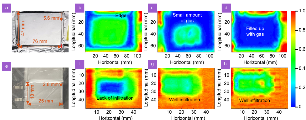
Fig. 5 | (a) Photograph of the LFP||Gr battery. The ultrasound image of the (b) healthy battery, (c) battery cycled for 2000 times and (d) faulty battery. (e) The photo of the AFLMB. (f) The ultrasound image of the dry AFLMB. The ultrasound images of the AFLMB when it is injected with electrolyte after (g) 24 hours and (h) 48 hours.
