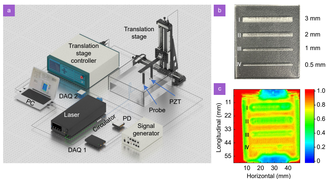
Fig. 4 | (a) The schematic diagram of the fiber optic ultrasound BHM system setup. (b) The photograph of the acrylic plate. (c) The imaging result of the acrylic plate.
