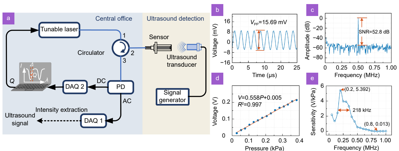
Fig. 2 | (a) The schematic diagram of the ultrasound sensing demodulation system. Detected signals when the voltage frequency is 500 kHz in (b) time domain and (c) frequency domain. (d) The output voltages of the sensor when ultrasound with different pressure is applied. (e) The frequency response of the sensor.
