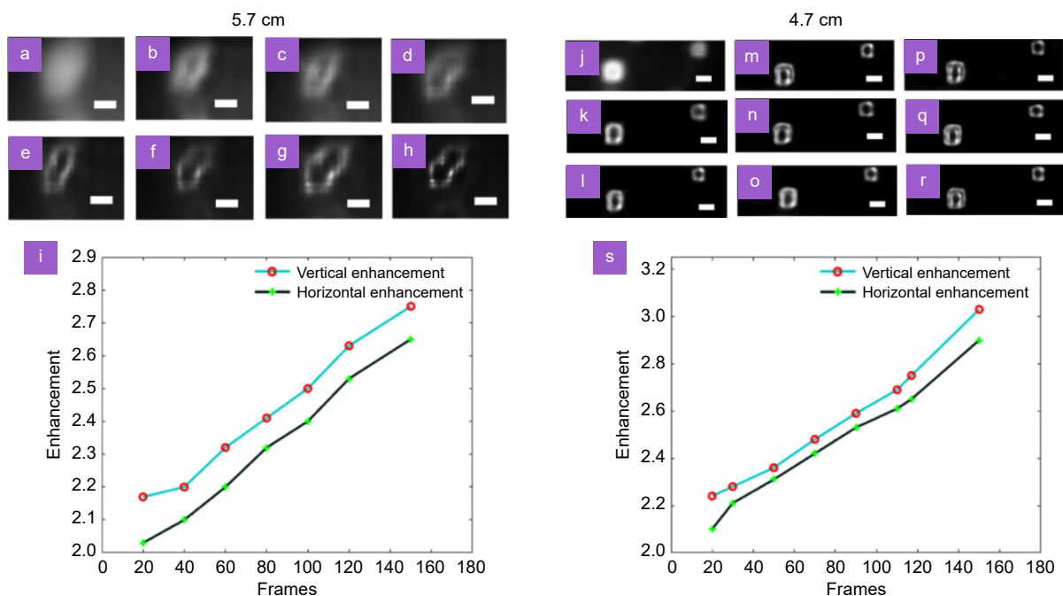
Fig. 6 | Sampling parameter vs enhancement. (a) Diffraction limited image. (b–h) Number of frames taken for SSIE processing: 20, 40, 60, 80, 100, 120, 150. Imaging distance: 5.7 cm, Scale bar: 200 μm. (j) Diffraction limited image. (k–r) Number of frames taken for SSIE processing: 20, 30, 50, 70, 90, 100, 110, 117, 150. Imaging distance: 4.7 cm, Scale bar: 600 μm. (i) Enhancement plot of (b–h). (s) Enhancement plot of (k–r).
