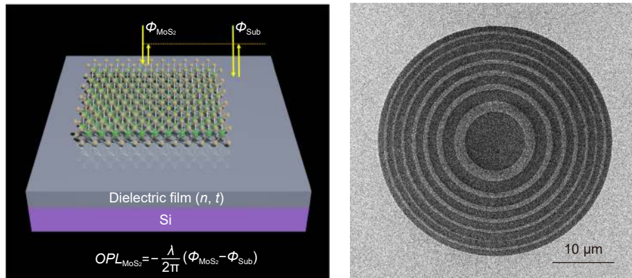
Atomically thin Fresnel zone plate with binary phase configuration
