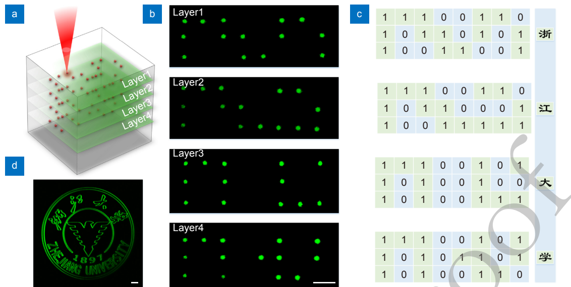
Fig. 3 | Optical information writing and readout. (a) Schematic diagram of 3D information writing in the glass. (b) Recorded information in glass in different layers. Dots in layer 1 and layer 2 are written by single pulse with 200 nJ. Dots in layer 3 and layer 4 are written by single pulse with 250 nJ and 300 nJ, respectively. Scale bar: 10 \mu\text{m} . (c) Encode information by binary format. (d) Complicated logo pattern recorded in the glass. Scale bar: 20 \mu\text{m} .
