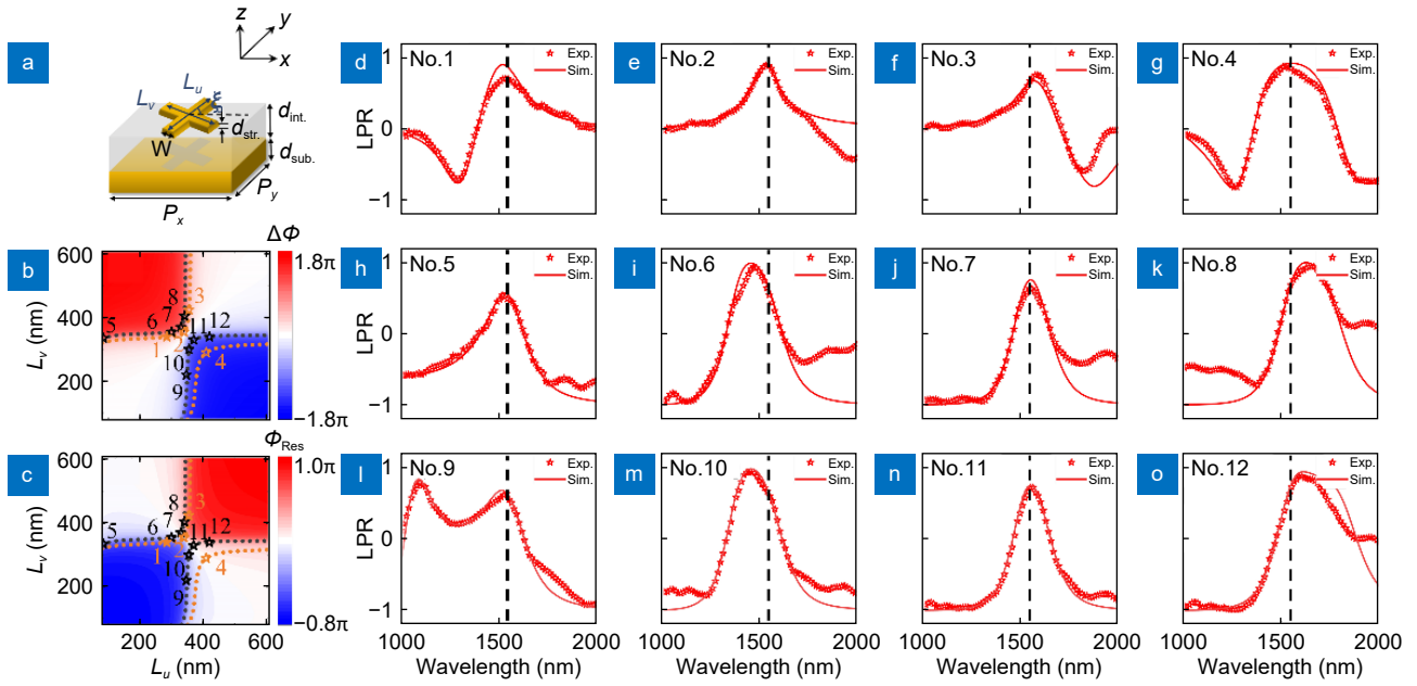
Fig. 2 | Schematic, phase diagrams and experimental characterizations of metaatoms. (a) Schematic of the designed metal-insulator-metal meta-atom with geometric parameters d_{\text{Str}} = 30 nm, d_{\text{Sub}} = 120 nm, d_{\text{Int}} = 120 nm, w = 80 nm, and P_x = P_y = 625 nm fixed. FDTD-simulated (b) phase difference \Delta\Phi and (c) resonant phase \Phi_{\text{Res}} of metaatoms with different L_u and L_v at the wavelength of 1550 nm. Orange dashed lines denote the cases \Delta\Phi = 0.5\pi and -1.5\pi and black dashed lines denote the cases \Delta\Phi = \pm\pi . Orange and black stars represent metaatoms labelled as Nos. 1–4 (functioning as QWPs) and Nos. 5–12 (functioning as HWPs), correspondingly. Experimentally measured LPR spectra of metaatoms (d) No.1, (e) No.2, (f) No.3, (g) No.4 under the RCP incidence and metaatoms (h) No.5, (i) No.6, (j) No.7, (k) No.8, (l) No.9, (m) No.10, (n) No.11, (o) No.12 under the incidence of LP light polarized along the angle 135^\circ . Dashed lines denote the positions of 1550 nm.
