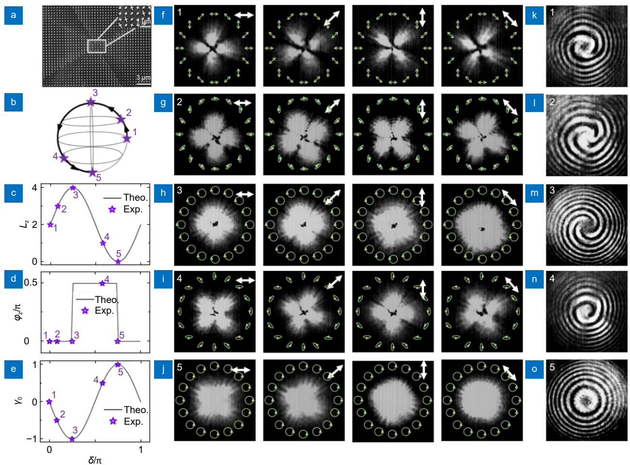
Fig. 4 | Experimental characterizations on metadvice II with incident polarization changing along path-I on the Poincare's sphere. (a) SEM image of the fabricated sample and a zoom-in picture (inset). (b) Path-I on the Poincare's sphere on which the incident polarization varies, with 1, 2, 3, 4 and 5 denoting five incident polarization states adopted for experimental characterizations. Theoretically calculated (line) and experimentally measured (stars) values of (c) L_z (d) \varphi_0 and (e) \gamma_0 versus the parameter \delta , which is the relative angle between a linear polarizer and a QWP employed in experiments to generate the desired incident polarization state. Measured intensity patterns of light reflected by our metasurface, under the illuminations of light at 1550 nm with polarizations with number (f) 1, (g) 2, (h) 3, (i) 4, and (j) 5 on the Poincare's sphere as shown in (b), with a rotatable polarizer placed in front of the detecting CCD tiled at the angles indicated by the white double-head arrows shown in right-up corners of each panels. Green symbols (arrows/circles/ellipse) illustrate the theoretically predicted polarization distributions in different cases. (k–o) Measured interference patterns between a spherical wave and the waves reflected by the metasurface, as shined by normally incident light at 1550 nm with polarizations corresponding to those 5 points on the Poincare' sphere as shown in (b).
