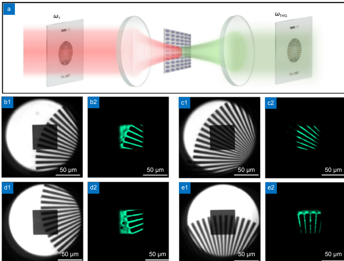
Fig. 1 | THG imaging based on Si membrane metasurfaces: the near-infrared signal passes through the target, then being converted into the visible signal via the metasurfaces, forming the target image on the CCD camera. (b1–e1) The images of the target and the metasurfaces under white light source illumination. (b2–e2) Transformed visible images of the target via membrane metasurfaces under NIR light illumination.
