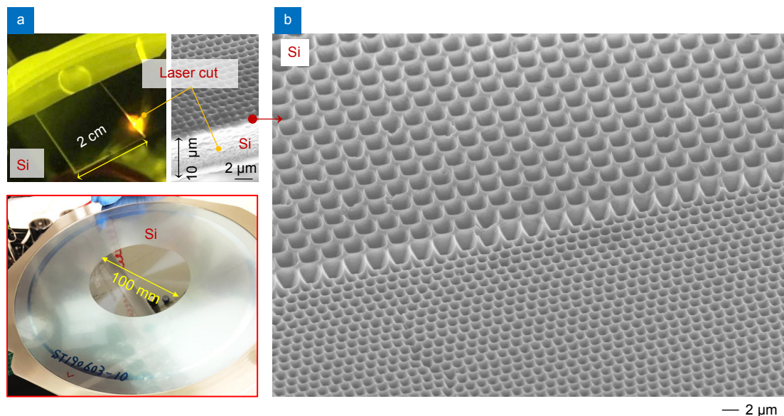
Fig. 4 | (a) 10- \mu\text{m} -thick Si wafer cut by E_p \approx 0.8 \text{ }\mu\text{J} energy fs-laser pulses (1030 nm/230 fs/200 kHz) using NA = 0.14 objective lens at 1 cm/s scan speed (5 passes with focus on the surface). SEM image of the 10- \mu\text{m} -thick Si wafer after cutting and patterning. Optical image of the 100-mm-diameter Si wafer on a plastic film. (b) PhC surface etched through holes ablated by fs-laser to define the Cr etch mask; NA = 0.9 lens was used, write speed 10 cm/s, pulse energy 12 nJ, laser repetition rate 200 kHz. Note the step height between regions with different period \Lambda . This step change is due to the under etch which is also responsible for formation of the upward-pyramid shown in inset of Fig. 3(b).
