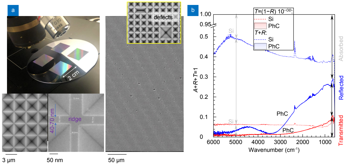
Fig. 6 | (a) Photo of large 2 × 2 cm 2 light trapping PhC patterns KOH etched through a chromium-mask defined by EBL; period \Lambda = 3.1 \mu\text{m} . SEM images of the final PhC pattern on 500-μm-thick n-type Si(100) wafer. (b) Color-coded presentation of portions of the absorbed A , reflected, R (measured) and transmitted T = (1 - R)10^{-0D} (measured) light at different wavelengths from 1.67 to 25 μm (or 6000–400 cm -1 in wavenumbers \bar{\nu} = 1/\lambda ).
