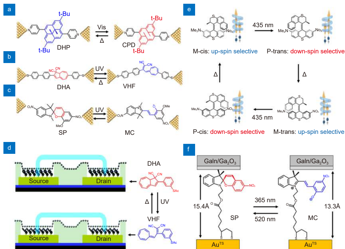
Fig. 3 | Other units used in single-molecule switches. (a) DHP/CPD single-molecule junction. (b) DHA/VHF single-molecule junction. (c) SP/MC single-molecule junction. (d) Schematic diagram of a vertical tunneling molecular switch with rGO thin films as the transparent top contact and the molecular structures of DHA and VHF. (e) Single-molecule switches with chirality molecules. The spin-polarization direction of the current switches with the chirality inversion. (f) Schematic diagram of SP SAMs in EGaIn/Ga 2 O 3 /SAM/Au TS junctions in their open and closed forms. Figure reproduced with permission from: (a) ref. 39 , American Chemical Society; (b) ref. 40 , under a Creative Commons Attribution 4.0 International License; (c) ref. 41 , American Chemical Society; (d) ref. 43 , John Wiley and Sons; (e) refs. 19,44 , under a Creative Commons Attribution 4.0 International License; (f) ref. 42 , American Chemical Society.
