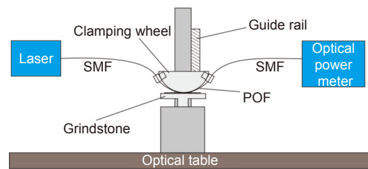
Fig. 6 | Schematic of experimental setup for polishing fibers.
