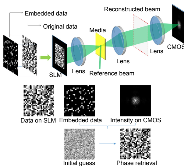
Fig. 9 | The diagram of non-interferometric system for phase retrieval based on IFT algorithm.
