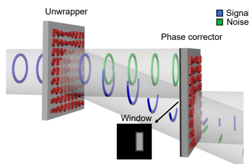
Off-axis cascade metasurface OAM demultiplexing system.
