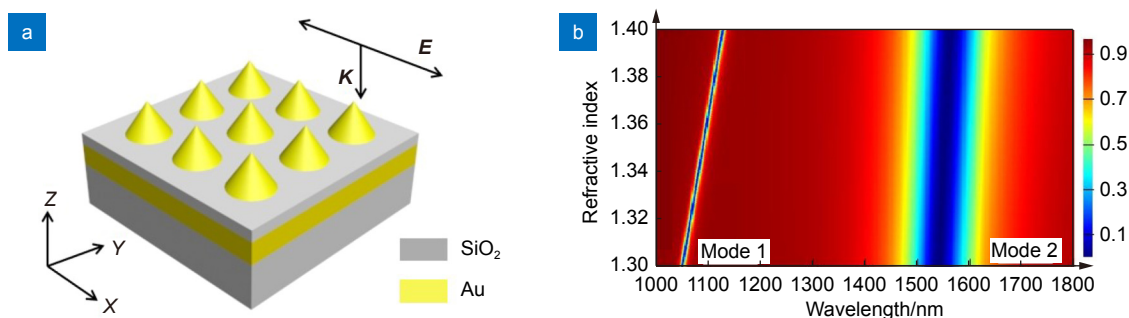
(a) Three dimensional schematic diagram of composite structure of Au nano cone and Au nano film;
