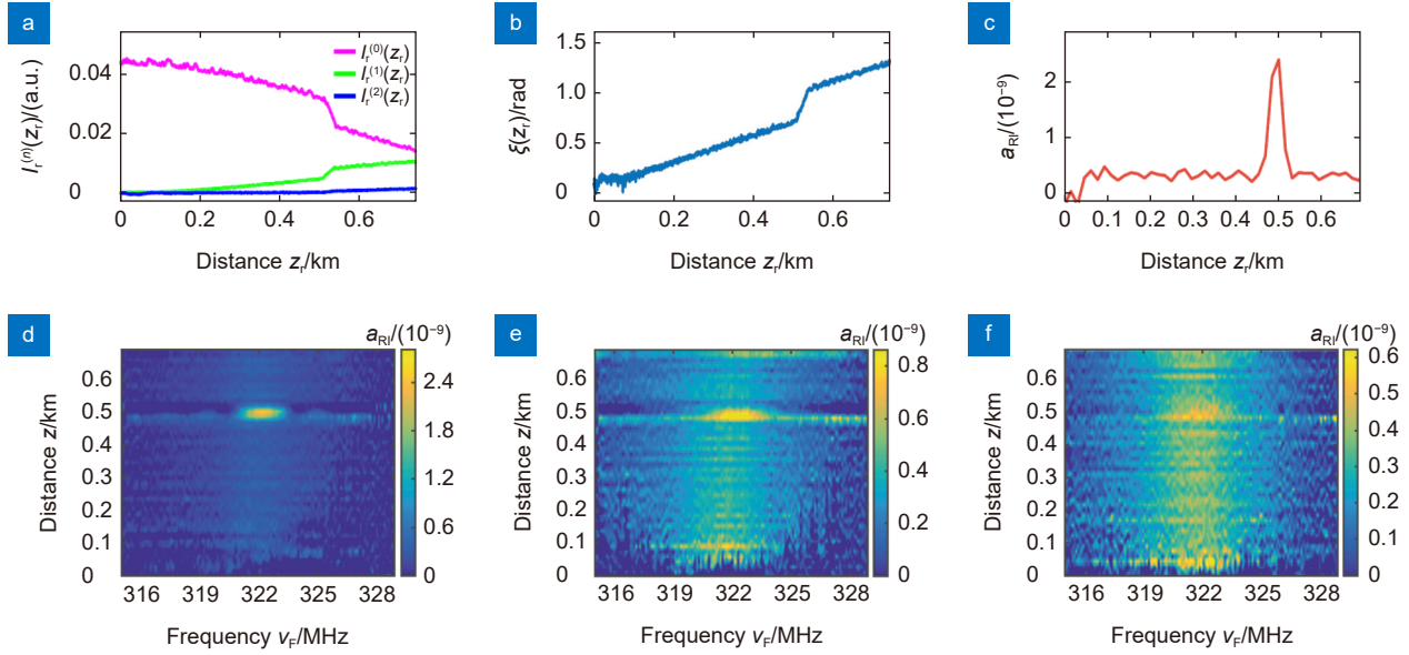
图 12 信号处理过程与实验结果。(a) 测量得到各阶边带光强的空间分布情况;(b) 还原出相位调制随距离的累积情况;(c) 微分得到的分布式相移结果;(d)~(f) 待测光纤置于空气、酒精和水中的测得的分布式 F-SBS 谱 [36] Fig. 12 Distributed F-SBS sensor based on local light phase recovery. (a) Distributed light intensity of 0, +1 and +2-order sidebands; (b) Phase accumulation along the fiber; (c) Distributed phase shift demodulated by differentiation; (d)~(f) Distributed F-SBS spectrums measured when the fiber under test placed in air, ethanol, and water [36]
