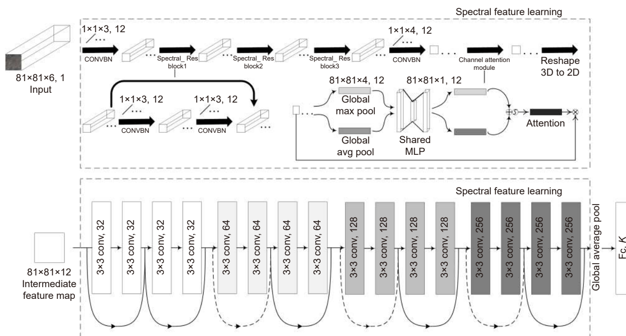
图4 残差3D-2D卷积神经网络
