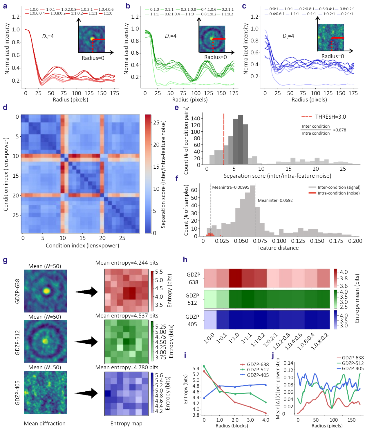
Fig. 3 | Hardware-level analysis of GDZP optical responses under spectral challenges. (a–c) Angle-averaged radial intensity profiles for GDZP-638, GDZP-512, and GDZP-405 under 10 distinct spectral challenges, demonstrating spectral-dependent spatial modulation induced by spectral excitation. (d–f) Condition-wise separability analysis accounting for repeatability noise, including the separability matrix, distribution of inter-/intra-normalized separation scores, and comparison of inter-condition and intra-condition feature distances. (g) Representative condition-mean diffraction patterns ( N = 50 ) under a balanced spectral challenge (1:1:1) and the corresponding block-wise entropy maps, illustrating the translation from a spatial structure to information content. (h) Lens-wise mean entropy across spectral challenges, highlighting challenge-dependent modulation of response statistics. (i) Radial entropy profiles extracted from the entropy maps, revealing annularly distributed information content. (j) Radial sensitivity curves quantifying the mean absolute change in radial intensity profiles between adjacent spectral challenges, identifying spatial regions with maximal challenge-induced modulation.
