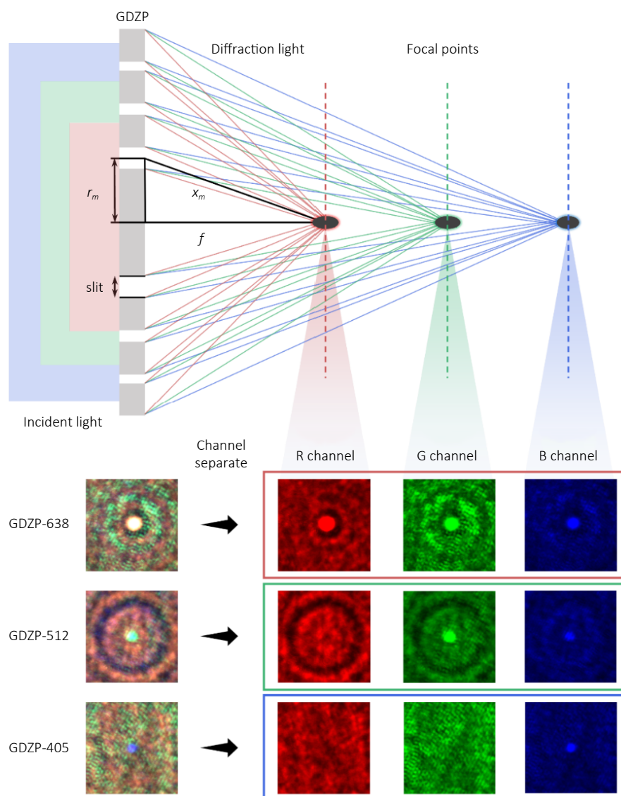
Fig. 2 | Operating principle and wavelength-dependent focusing behavior of GDZPs. The schematic illustrates the planar diffractive mechanism based on Fresnel zone plate theory, in which concentric graphene zones modulate the incident wavefront to produce constructive interference at a focal distance f . Because the GDZP is diffractive, the focal position exhibits negative chromatic aberration, shifting systematically with illumination wavelength. Three GDZPs designed for wavelengths of 638, 512, and 405 nm were fabricated to share an identical focal length of f=220\ \mu\text{m} . Diffraction patterns were recorded at a fixed observation plane under identical RGB mixed-laser illumination with equal power in each channel. Channel-separated images show that each GDZP produces a pronounced focal response primarily in the channel corresponding to its design wavelength, whereas non-matching wavelengths exhibit defocused or low-contrast patterns.
