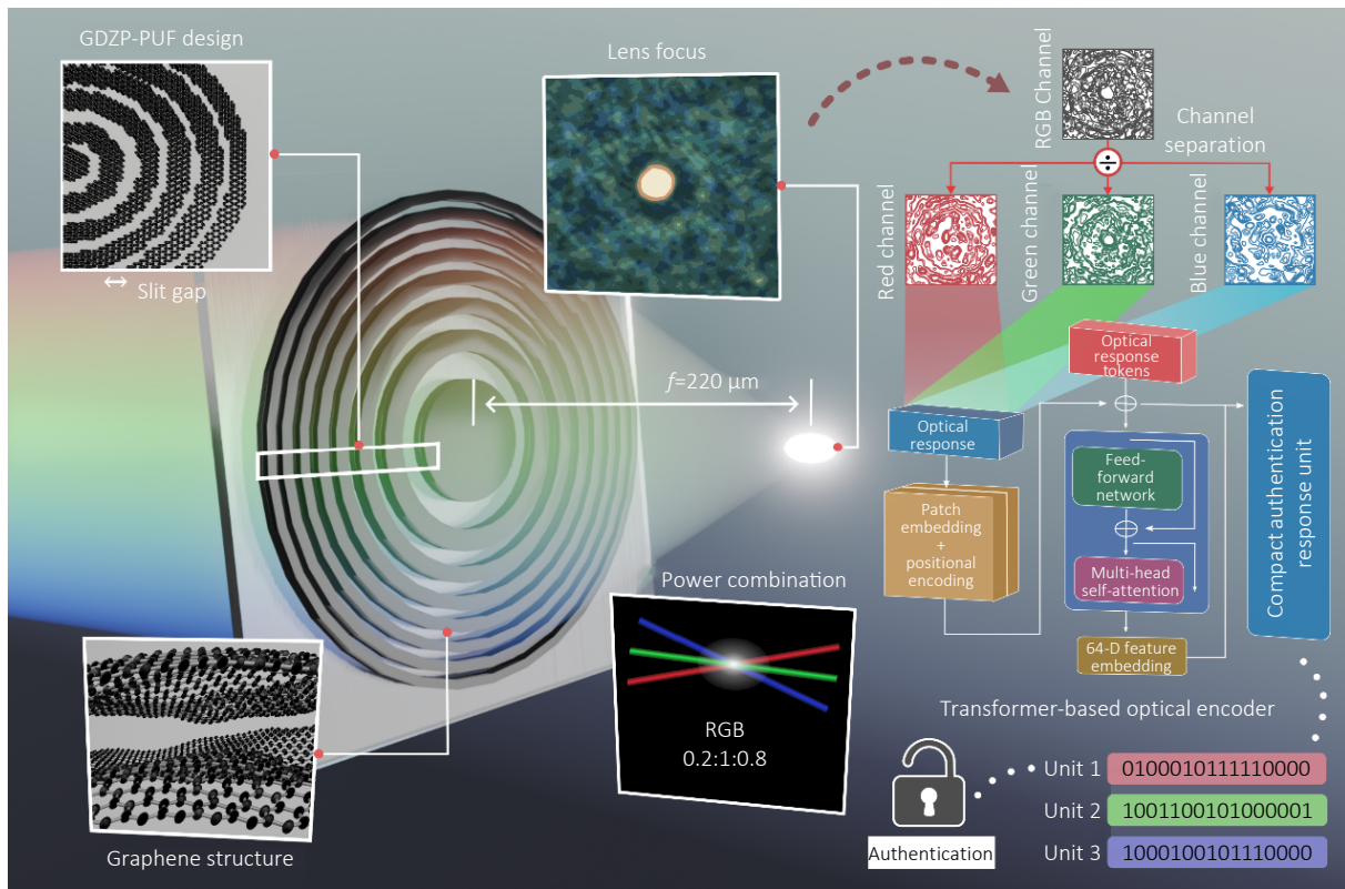
Fig. 1 | Overview of the GDZP-ViT optical PUF system. The system combines a structured GDZP diffractive front-end with a learning-based processing pipeline to convert raw diffraction responses into compact, analyzable representations. The GDZP response arises from the coexistence of deterministic Fresnel-zone-plate diffraction and microscopic graphene-induced disorder, while controlled multi-wavelength excitation modulates the optical response through wavelength-dependent dispersion. The resulting RGB diffraction patterns are captured by a CMOS sensor and processed by a ViT to extract compact embeddings used for subsequent PUF analysis.
