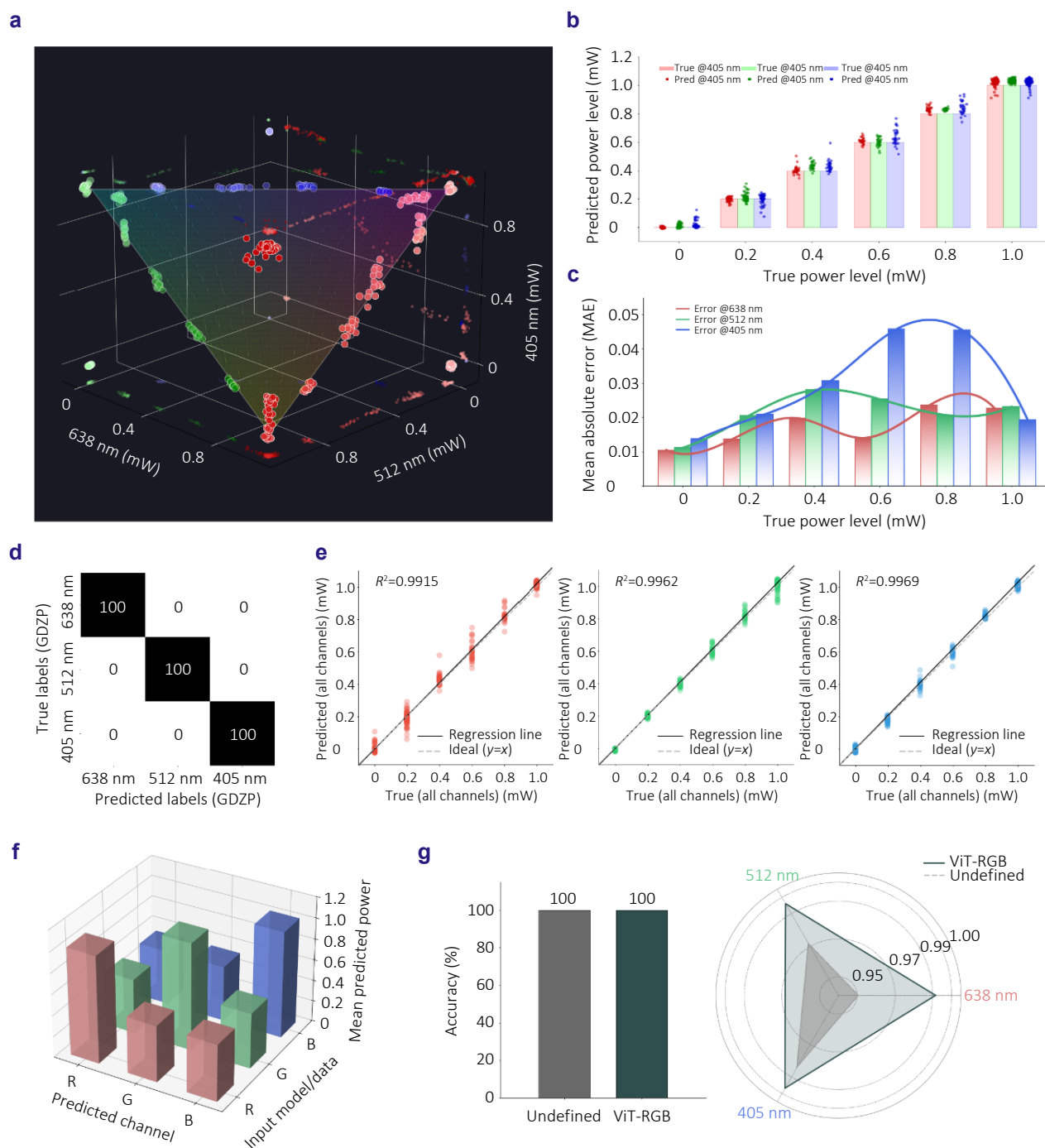
Fig. 5 | Evaluation of ViT-learned optical embeddings and their suitability for PUF authentication. (a) Three-dimensional embedding of decoded RGB spectral conditions, illustrating that responses measured under identical challenges cluster tightly in the learned space. (b) Distribution of decoded spectral values across discrete power levels, demonstrating consistent embedding stability over the full dynamic range. (c) MAE of decoded spectral parameters as a function of power level, reflecting low intra-condition variation. (d) Confusion matrix for GDZP design-class identification, indicating strong configuration-level separability in the embedding space. (e) Linear correspondence between decoded and nominal spectral parameters, confirming monotonic and thresholdable embedding behavior. (f) Cross-channel attribution matrix showing effective disentanglement of wavelength-dependent responses. (g) Comparison with a baseline CNN, highlighting the advantage of global context-aware representations for stable optical embedding.
