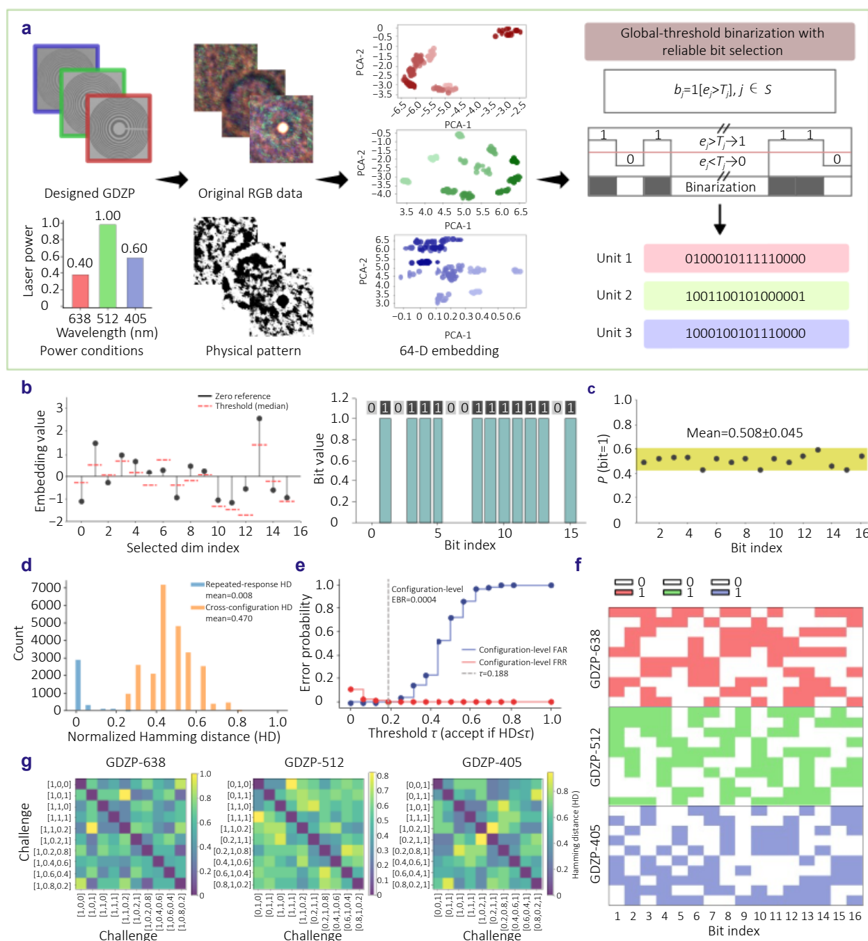
Fig. 6 | Binary response extraction and authentication performance of the GDZP-VIT optical PUF system. (a) Overview of the binary response extraction pipeline. Designed GDZPs under controlled spectral challenges generate raw RGB diffraction patterns, which are transformed into 64-dimensional learned embeddings and subsequently binarized via median thresholding with reliability-driven bit selection to produce 16-bit binary response units. Each response unit corresponds to a single spectral challenge and serves as a compact building block for constructing longer authentication tokens, rather than as a standalone 128-bit or 256-bit cryptographic key. (b) Illustration of dimension-wise binarization by comparing embedding values with median thresholds. (c) Bit uniformity analysis showing the probability of bit value "1" across selected dimensions. (d) Distributions of repeated-response and cross-configuration normalized HDs. The repeated-response HD quantifies measurement repeatability under the same GDZP design and spectral challenge, whereas the cross-configuration HD quantifies separability across the tested GDZP design/challenge configurations. (e) Threshold-dependent estimated FAR and FRR derived from empirical threshold sweeping of the repeated-response and cross-configuration HD distributions in (d), without parametric curve fitting. The resulting EER represents a configuration-level separability estimate for the present dataset. (f) Visualization of representative binary response units across different GDZP designs and spectral challenges. (g) Inter-condition HD matrices for each GDZP design, validating challenge-dependent response diversity across the experimentally tested spectral conditions.
