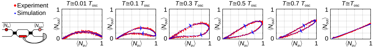
Fig. 3 | Experimental and simulation results for the hysteresis loop of a single photonic quantum memristor with different ratios between the two time scales: oscillation period of the modulated input flux, T_{\text{osc}} , and time length of the memristor's buffer, T . On the left, a schematic diagram of the device is shown. For non-zero area, blue triangles show the direction of the hysteresis loops with respect to the sweep of the input photon number. Being small, error bars are neglected here for clarity. The raw data are affected by 1%–5% relative error.
