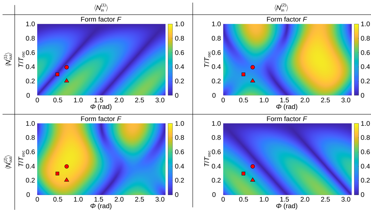
Fig. 5 | Simulations of the form factor F of the intra- and inter-memristor hysteresis curves of two coupled photonic quantum memristors with crossed feedbacks as a function of the relative phase \Phi between their inputs and the ratio T/T_{\text{osc}} between the buffer length of the memristors, T , and the period of the sinusoidal input modulation, T_{\text{osc}} . The form factor F is 4\pi times the ratio between the area and the squared perimeter of the hysteresis curve. The intra-relations, (\langle N_{\text{in}}^{(1)} \rangle, \langle N_{\text{out}}^{(1)} \rangle) and (\langle N_{\text{in}}^{(2)} \rangle, \langle N_{\text{out}}^{(2)} \rangle) , are on the diagonal of the table, and the inter-relations, (\langle N_{\text{in}}^{(2)} \rangle, \langle N_{\text{out}}^{(1)} \rangle) and (\langle N_{\text{in}}^{(1)} \rangle, \langle N_{\text{out}}^{(2)} \rangle) , are on the off-diagonal. The values have been normalized with respect to the maximum value of F for the inter-relations, i.e. \approx 0.95 for T/T_{\text{osc}} \approx 0.5 and relative phases \Phi \approx 2.35 rad and \Phi \approx 0.77 rad, respectively. The red symbols in the surface plots indicate the choice of parameters used in the experiments of the two coupled memristors with crossed feedback reported in Fig. 4: in particular, the triangle-square-circle represents the choice associated with the hysteresis curves in Fig. 4(b–d), respectively.
