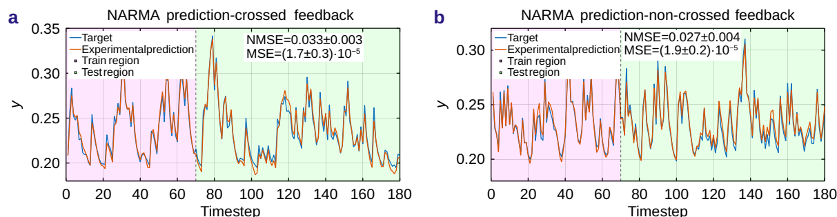
Fig. 7 | Experimental prediction of NARMA time series using coupled memristors with (a) crossed and (b) non-crossed feedback laws. NARMA is defined as y(t+1) = 0.4y(t) + 0.4y(t)y(t-1) + 0.6x^3(t) + 0.1 , x(t) being a uniformly distributed random number in the interval [0, 1/2] 42 . The modulation of \langle N_m^{(1)}(t) \rangle (via MZI-1) is x^2(t) , while an additional \pi/5 phase shift is applied to MZI-2. The reflectivity update follows a moving-average-like feedback law: R^{(i)}(t) = R^{(i)}(t-1) + [\langle N_m^{(j)}(t-1) \rangle - R^{(i)}(t-1)]/M^{(i)} , where i=[1, 2] and j can be equal (non-crossed feedback) or different (crossed feedback) to i . The acquired datasets are split into a training stage and a test stage. In the training stage, a linear regression of output photon fluxes ( X ) to y is performed to obtain the coefficients w such that y = w \cdot X . Then, the same coefficients w are applied to the outputs in the test stage to predict the function. In the plots, the 'experimental prediction' is y_{\text{pred}} = w \cdot X , which is an effective prediction only in the test stage. To assess the quality of the prediction, we estimate both the mean squared error ( \text{MSE} = \sum (y - y_{\text{pred}})^2 / N ) and the normalized MSE ( \text{NMSE} = \text{MSE} / \text{var}(y) ) over the test region. The two estimators are reported with their uncertainties obtained by statistics on 5 datasets. The \pi/5 phase shift and the values of M^{(1)}=3 , M^{(2)}=4 for both feedback cases were chosen after performing simulations. These experiments have been performed with an attenuated CW laser with wavelength 750 nm.
