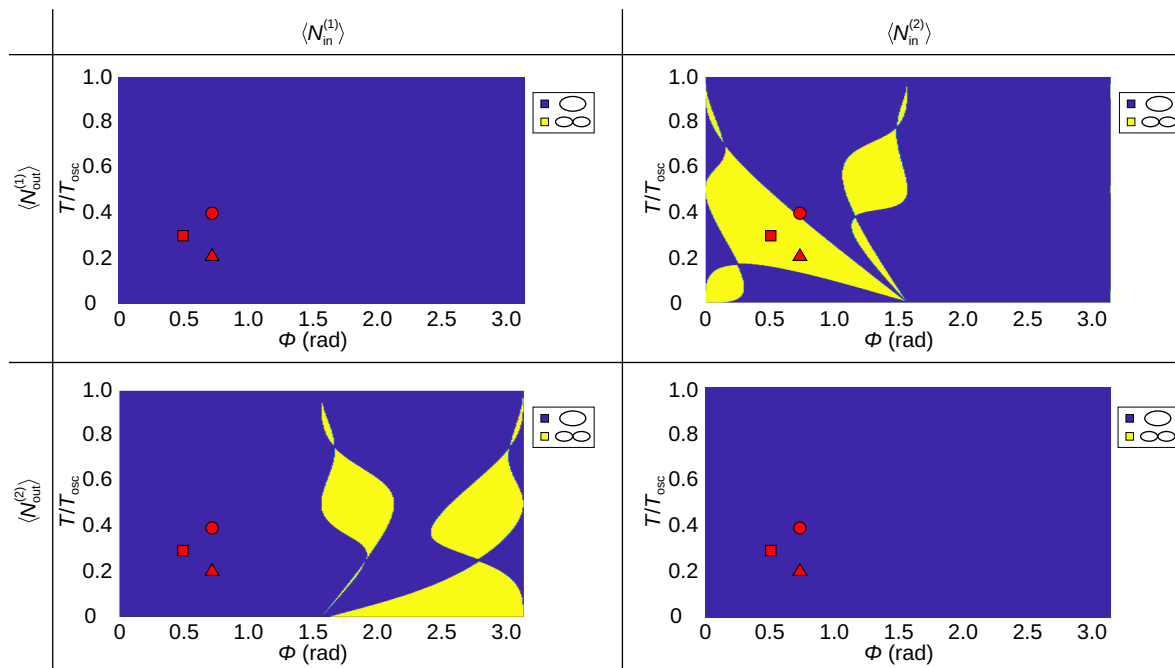
Fig. 6 | Simulations results revealing the presence (yellow regions) of a self-intersecting hysteresis loop in two coupled PQMs with crossed feedback as a function of the relative phase \Phi between the inputs and the ratio T/T_{osc} between the buffer length of the memristors, T , and the period of the sinusoidal input modulation, T_{osc} . The infinity symbols and the yellow stands for self-intersecting curves, while the ellipse and the blue for not-self-intersecting curves. The red symbols in the surface plots indicate the choice of parameters used in the experiments of the two coupled memristors with crossed feedback reported in Fig. 4: in particular, the triangle-square-circle represents the choice associated with the hysteresis curves in Fig. 4(b–d), respectively.
