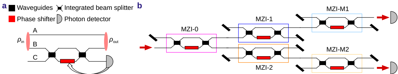
Fig. 2 | (a) Dual-rail scheme of the photonic quantum memristor, where the input state \rho_{\text{in}} is encoded as a single photon in a superposition of the upper path modes A-B. The component in mode B is transformed by the Mach-Zehnder interferometer, implementing the photonic quantum memristor, while the component in mode A propagates freely to the output state \rho_{\text{out}} . The Mach-Zehnder interferometer is composed of two beam splitters (black rectangles), and a thermal phase shifter (red rectangle). The output on mode C is used as a feedback for the phase setting of the memristor. (b) Schematic layout of the circuit implementing a single (MZI-M1) and two coupled integrated photonic quantum memristors (MZI-M1 and MZI-M2). The red arrow on the left indicates the input waveguide, while the arrows on the right are placed to highlight the output waveguides, fiber-coupled to single-photon SPAD detectors, which are represented by grey semi-circles. MZI-0, MZI-1, MZI-2 are used to prepare the suitable input state for the PQM. The input and output waveguides that are not used in the experiments are pointed out by a black oblique line.
