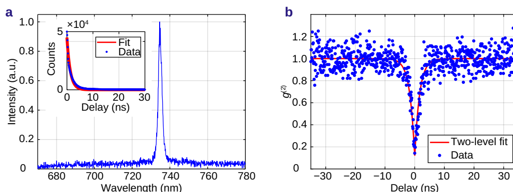
Fig. 1 | (a) The photoluminescence spectrum of the \text{SiV}^- showing a sharp ZPL peak at 734 nm. In the inset, the time decay of the photoluminescence (points) and its single exponential fit (line). The fit yields a lifetime of the \text{SiV}^- of 1.89 ns. (b) Second order correlation data (points) of the emitted photons as a function of the time delay between the two arms of the HBT interferometer. Data are fitted by a two levels model (line) which evidences a clear photon antibunching behaviour.
