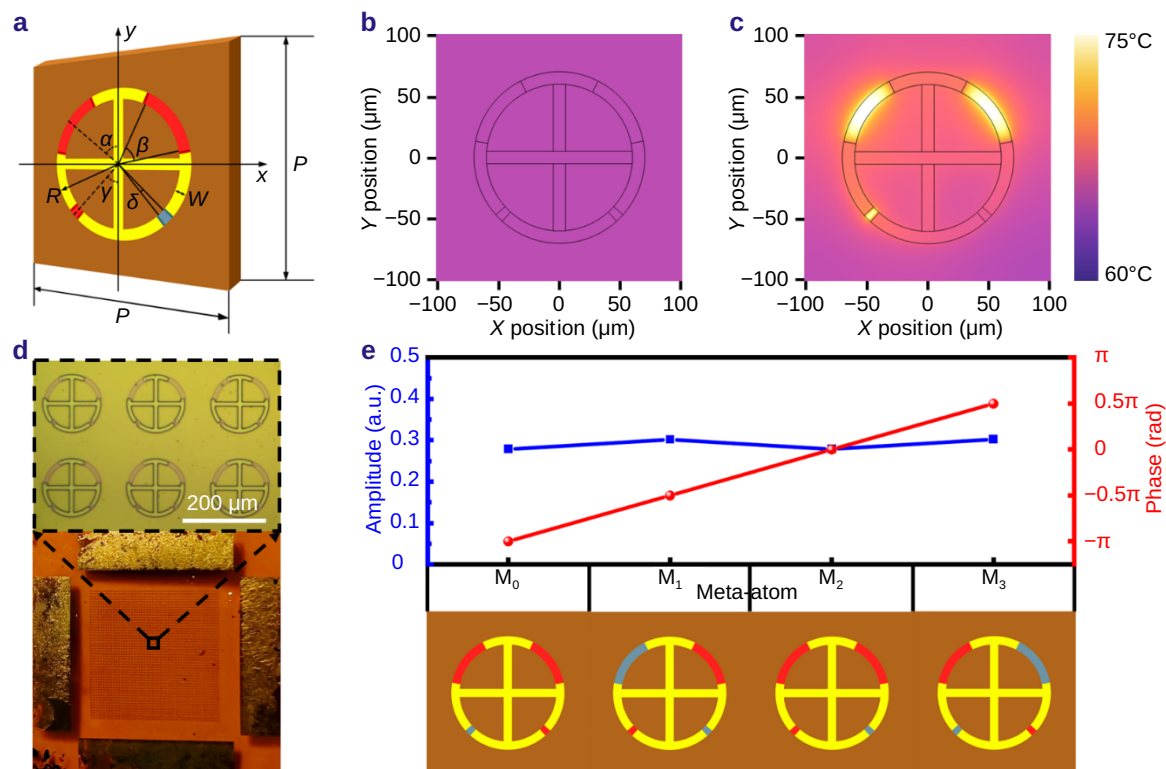
Fig. 2 | Design of the meta-atom in the programmable metasurface. (a) Schematic diagram of the V-CSRRs unit (meta-atom) with one gap containing a VO 2 patch at -45° in its insulating (gray) state and other gaps with VO 2 patches in their metallic (red) state. (b, c) Simulated thermal distributions for the meta-atom located on the Sapphire (b) and PI (c) substrate, respectively. (d) Optical photo of the successfully fabricated programmable metasurface. The inset displays a microscopic image of the sample, where the scale bar represents 200 μm. (e) Simulated cross-polarized transmission amplitude and phase responses of the proposed meta-atoms for four distinct coding states under normal incidence of an x -polarized THz wave at 0.7 THz. The insets illustrate the selective IMT configurations of the VO 2 patches for coding states M 0 –M 3 . Adjacent coding states yield nearly identical amplitude while introducing a phase increment of approximately \pi/2 .
