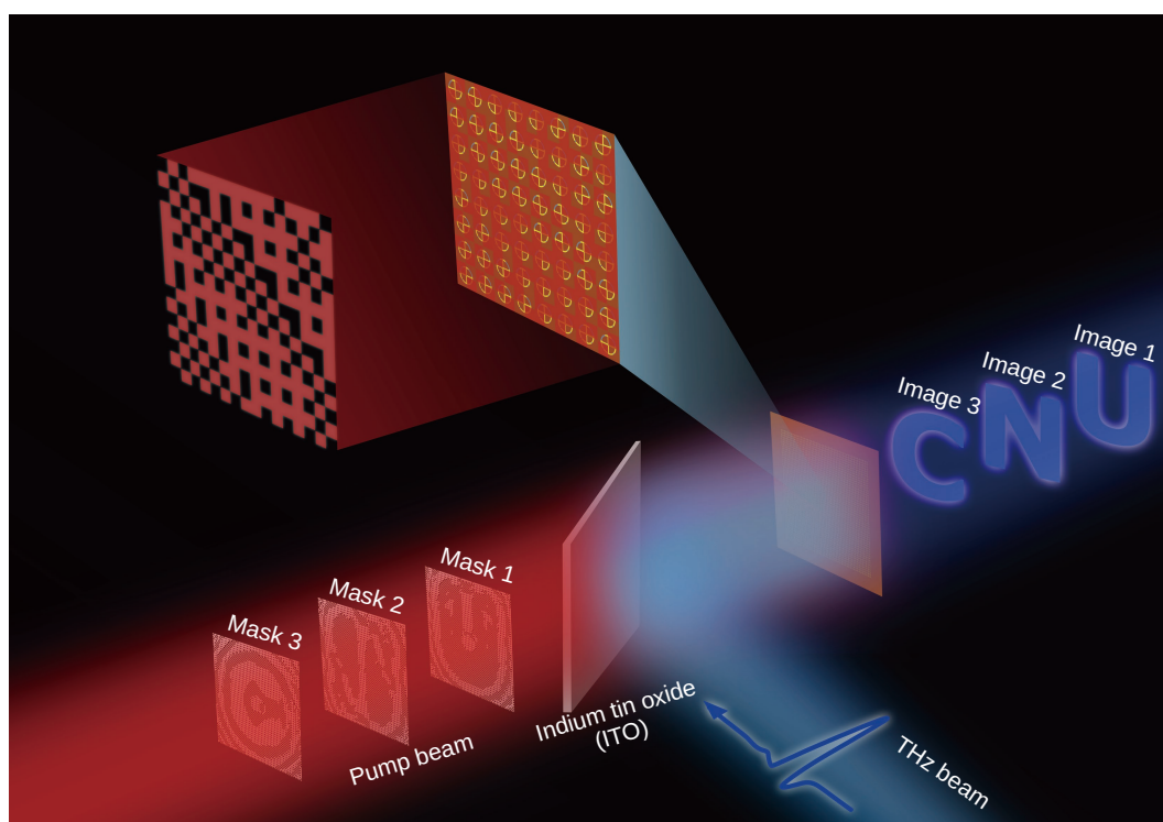
Fig. 1 | Schematic of the pixel-controlled programmable metasurface as a PSTM.
