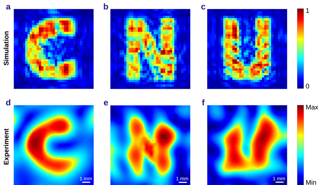
Fig. 5 | Experimental results of dynamic holographic imaging. (a–c) Theoretical expectations of letters “C”, “N” and “U” reconstructed by the GS algorithm, respectively. (d–f) Experimental results for measured holographic images of the letters “C”, “N” and “U” at 0.7 THz, respectively. The scale bar is 1 mm.
