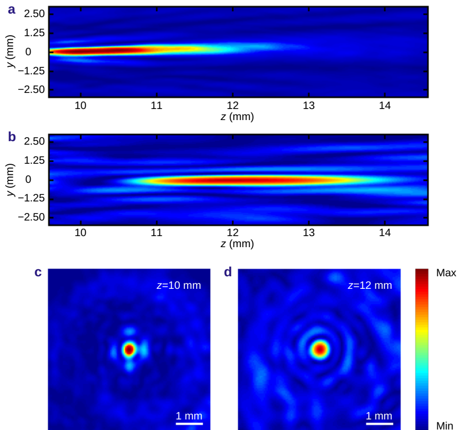
Fig. 3 | Experimental demonstration of the THz dynamic zoom meta-lens. (a, b) Experimental results of y -polarized THz electric field profile in the yz plane, when the metasurface (surface normal vector along z -direction) is illuminated with x -polarized THz waves, for the designed zoom meta-lens with focal lengths f_1 = 10 mm (a) and f_2 = 12 mm (b), respectively. (c, d) Measured results of the THz electric field intensity, extracted at the corresponding focal planes from (a) and (b), respectively.
