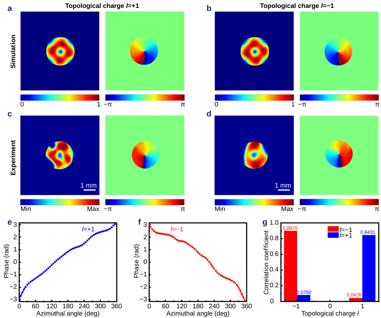
Fig. 4 | Generation of focused vortex beam with tunable topological charges. (a, b) Simulated normalized THz field intensity and phase distributions for topological charges l = +1 and l = -1 . (c, d) Intensity and phase distributions of the focused THz vortex beams at focal plane ( z = 11 mm) for the design frequency of 0.7 THz experimentally measured by optical-pump THz-imaging system for topological charges l = +1 and l = -1 . The scale bar is 1 mm. (e, f) Relationship between phase variation curves and azimuthal angle for l = +1 and l = -1 with the radial distance r = 0.8 mm. (g) Correlation coefficients of the experimentally measured focused vortex beams with different topological charges.
