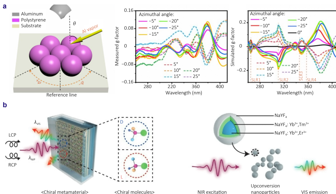
Fig. 15 | Nanoparticle-enhanced chiral sensing strategies. (a) Core-shell metamaterials based ultrasensitive ultraviolet chiral plasmonic biosensor. (b) Upconversion nanoparticles extending sensitivity from femtomolar to nonlinear detection regimes. Figure reproduced with permission from: (a) ref. 274 , American Chemical Society; (b) ref. 245 , Wiley-VCH GmbH.
