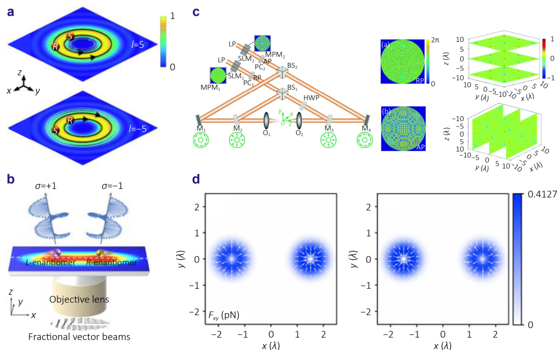
Fig. 7 | Structure light beams for enantioselective optical manipulation. (a) The optical separation and discrimination of chiral particles using the focused vector vortex beam carrying the orbital angular momentum. (b) Trapping chiral particles using tightly focused FVBs. (c) The 4\pi microscopic system integrated with MPMs encoded by phase-only SLMs for achieving a controllable chiral optical field. (d) Chirality-sorting optical force pairs generated in a tightly focused Gaussian beam by tailoring the input polarization state. Figure reproduced with permission from: (a) ref. 134 , under a Creative Commons Attribution-Non Commercial 3.0 Unported Licence; (b) ref. 137 , Optica Publishing Group; (c) ref. 138 , Royal Society of Chemistry; (d) ref. 139 , American Physical Society.
