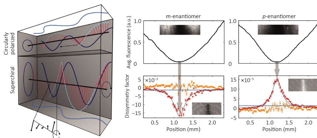
Fig. 11 | Early demonstration of superchiral light for enhanced chiral molecular detection. A standing-wave configuration formed by reflecting circularly polarized light from a mirror generates localized high-chirality hotspots, achieving an 11-fold sensitivity enhancement in chiral discrimination. Figure reproduced with permission from: ref. 49 , AAAS.
