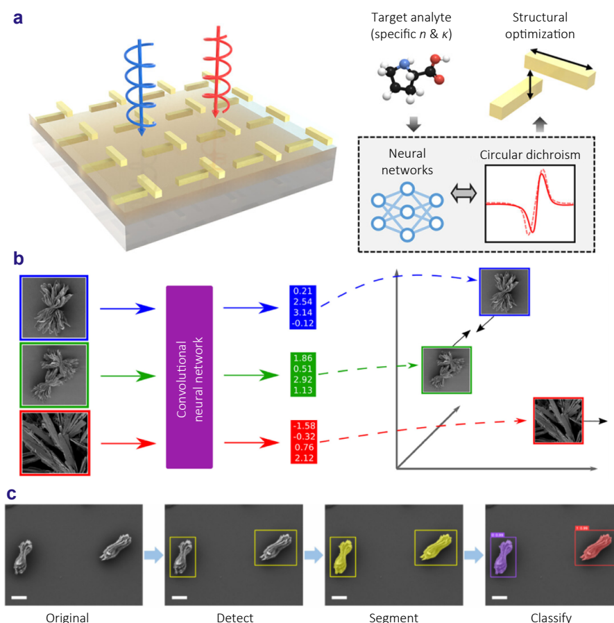
Fig. 17 | Artificial intelligence in chiral detection. (a) Neural network-guided genetic algorithms for optimizing plasmonic nanodimer sensors, enabling ultra-sensitive enantiomer discrimination. (b) Deep learning models employing Siamese architectures to identify nanoparticle handedness directly from SEM images. (c) Automated segmentation and classification pipelines integrating Grounding DINO, Segment Anything, and ResNet, achieving high-throughput and annotation-free analysis of chiral nanoparticles. Figure reproduced with permission from: (a) ref. 316 , American Chemical Society; (b) ref. 318 , American Chemical Society; (c) ref. 319 , American Chemical Society.
