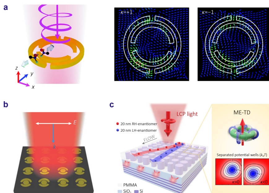
Fig. 9 | Metasurface-assisted chiral sorting via multipolar interference. (a) Plasmonic split-ring apertures enabling Fano-enhanced chiral forces. (b) Dipole-octupole Fano resonances generating strong enantioselective for sorting sub-10 nm particles. (c) Toroidal dipole metasurface producing enhanced forces in flowing liquid streams, demonstrating high-throughput enantioseparation. Figure reproduced with permission from: (a) ref. 151 , Royal Society of Chemistry; (b) ref. 152 , Wiley-VCH GmbH; (c) ref. 45 , American Chemical Society.
