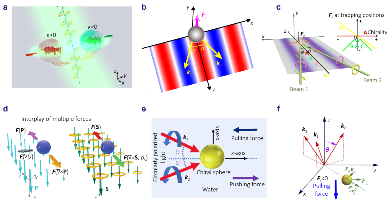
Fig. 6 | Optical lateral forces and optical pulling forces on chiral particles. (a) Separating chiral particles placed at the interface of air and water with a linearly polarized light wave. (b) Chiral sorting using a standing wave from two linearly polarized beams. (c) OLF on chiral particles resulted from a standing wave configured from two waves with different polarizations. (d) Observation of multiple-parameter chiral optical force on a chiral sphere in a spin-curl light field. (e) Chiral sorting by OPF generated from an interferential field constructed of two circularly polarized beams. (f) Chiral sorting by OPF generated from an interferential field composed of three circularly polarized beams. Figure reproduced with permission from: (a) ref. 92 , 2020 Springer Nature; (b) ref. 95 , American Physical Society; (c) ref. 96 , American Chemical Society; (d) ref. 129 , American Physical Society; (e) ref. 41 , Optica Publishing Group; (f) ref. 133 , Optica Publishing Group.
