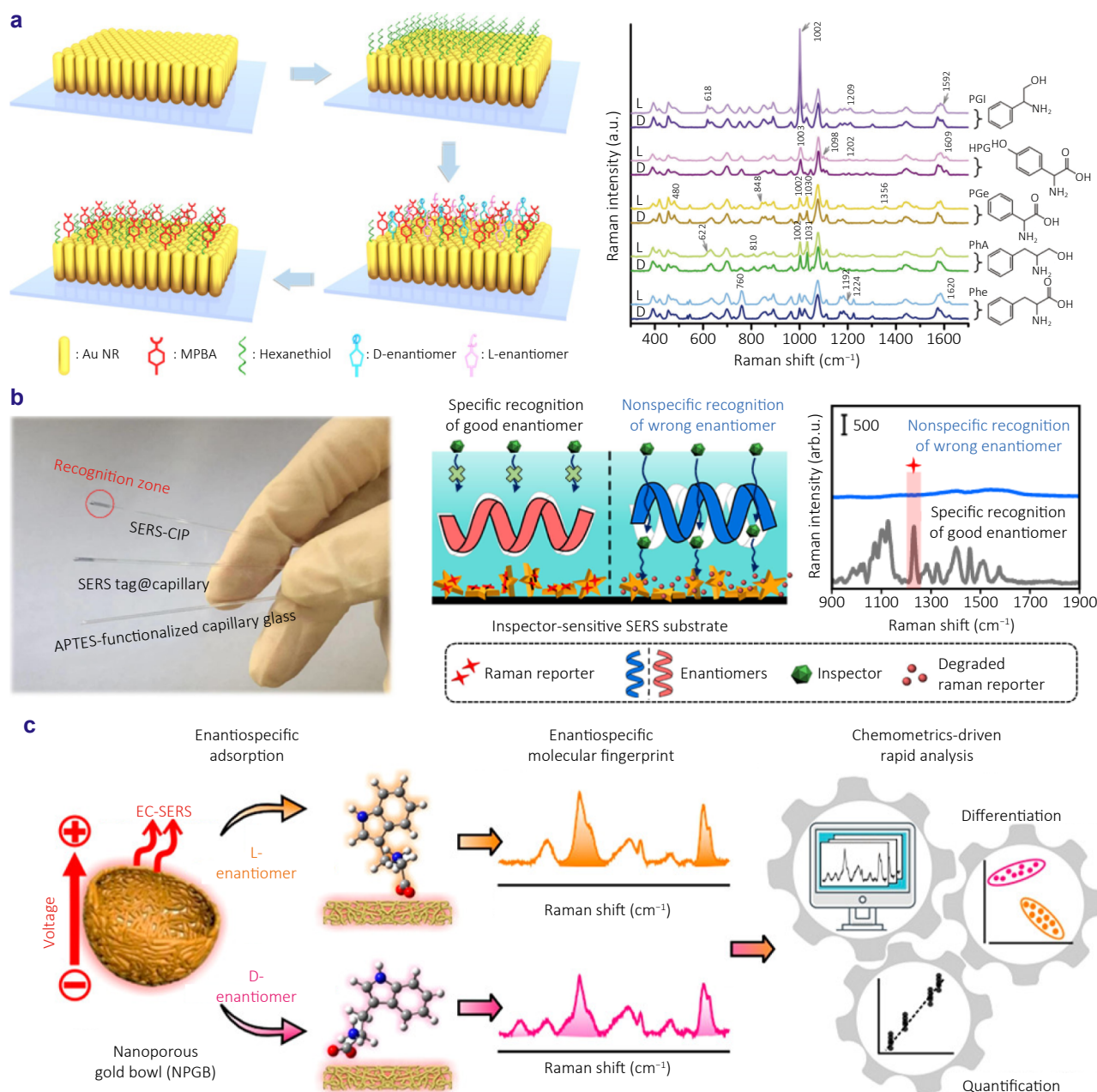
Fig. 16 | SERS-enabled chiral sensing strategies. (a) Label-free SERS using vertically aligned Au nanorod arrays for molecular enantiomer discrimination. (b) Chiral-imprinted polydopamine substrates combined with inspector molecules enabling absolute chiral discrimination with ultrahigh sensitivity. (c) Nanoporous gold bowls coupled with electrochemical modulation to realize stereospecific enantiomer absorption and molecular fingerprinting. Figure reproduced with permission from: (a) ref. 276 , Wiley-VCH GmbH; (b) ref. 277 , under a Creative Commons CC BY license; (c) ref. 278 , American Chemical Society.
