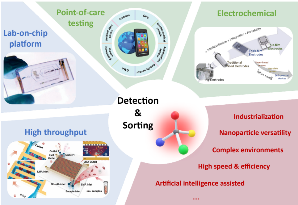
Fig. 18 | Schematic illustration of future prospects in chiral optical sorting and detection. For sorting, key directions include integration with microfluidic systems, development of lab-on-chip platforms 323 , and achieving high-throughput 328 enantioselective separation. For detection, research is advancing toward point-of-care testing 325 and hybrid multimodal strategies 327 for more efficient measurements. In addition, large-scale industrialization, broad nanoparticles versatility across diverse physical properties, adaptation to complex real-world environments, high speed and efficiency, and AI-assisted data analysis and the pursuit of faster, more reliable operation represent common goals for both sorting and detection. Figure reproduced with permission from: ref. 323 , Royal Society of Chemistry; ref. 325 , Wiley-VCH GmbH; ref. 327 , Elsevier B.V.; ref. 328 , Wiley-VCH GmbH.
