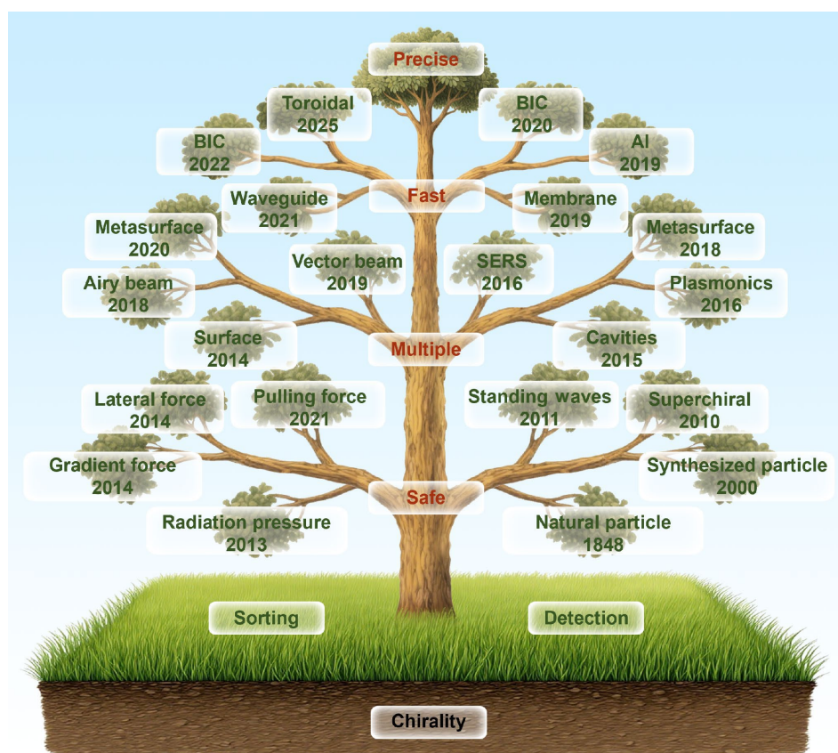
Fig. 2 | Chiral tree for the timeline of key milestones in optical sorting and detection. The left panel highlights the development of optical sorting, from early demonstrations of radiation pressure to gradient forces, lateral forces, and pulling forces, and more recent approaches involving structured beams, waveguides, and metasurfaces. The right panel summarizes advances in optical detection, from early circular dichroism of natural and synthesized chiral particles and the introduction of superchiral fields to plasmonics, nanocavities, metasurfaces, and AI-assisted chiral sensing.
