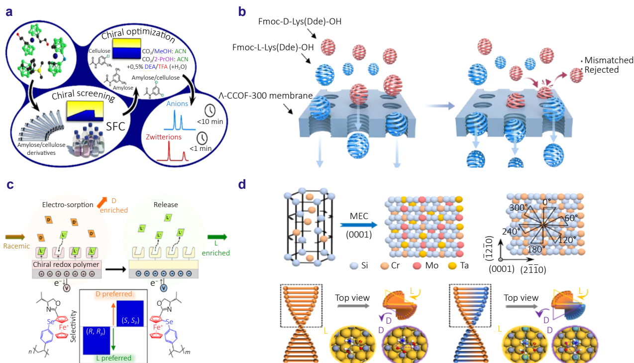
Fig. 3 | Representative chemical methods for enantioseparation. (a) Supercritical fluid chromatography with polysaccharide CSPs for efficient separation. (b) COFs-based membrane systems enabling size- and chiral-selective transport. (c) Redox-responsive planar-chiral metallopolymer enabling switchable enantioselective absorption. (d) Medium-entropy ceramics surfaces acting as chiral adsorbents via asymmetric binding energies. Figure reproduced with permission from: (a) ref. 77 , American Chemical Society; (b) ref. 71 , Springer Nature; (c) ref. 85 , American Chemical Society; (d) ref. 86 , Springer Nature.
