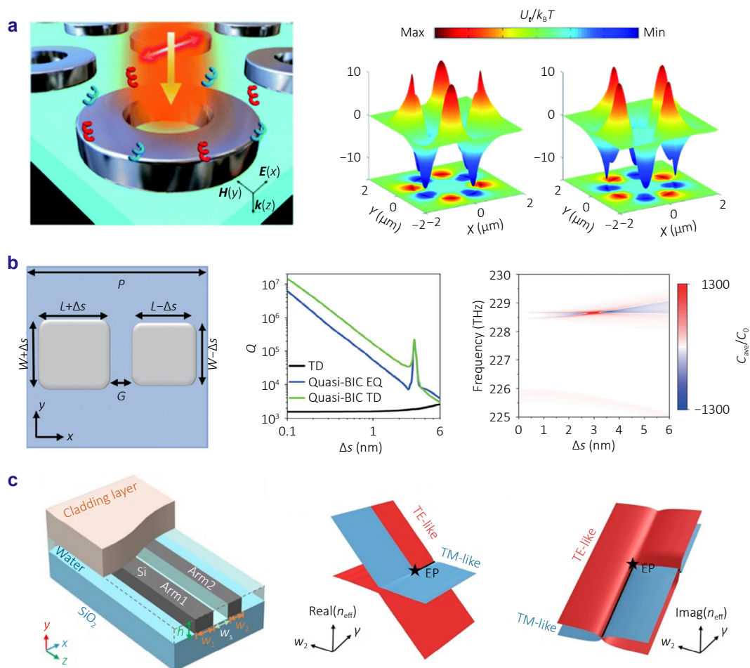
Fig. 10 | Novel metasurface physics for chiral sorting. (a) qBIC magnetic dipole resonance producing strong chirality density gradients for sub-2 nm particle separation. (b) Dual qBIC silicon dimers achieving near-perfect field overlap and 10^4 -fold superchiral enhancement. (c) Vector exceptional point metasurface integrated with microfluidics, generating powerful chiral gradient forces for efficient on-chip enantioseparation. Figure reproduced with permission from: (a) ref. 44 , Royal Society of Chemistry; (b) ref. 175 , American Physical Society; (c) ref. 179 , under a Creative Commons Attribution (CC BY) license.
