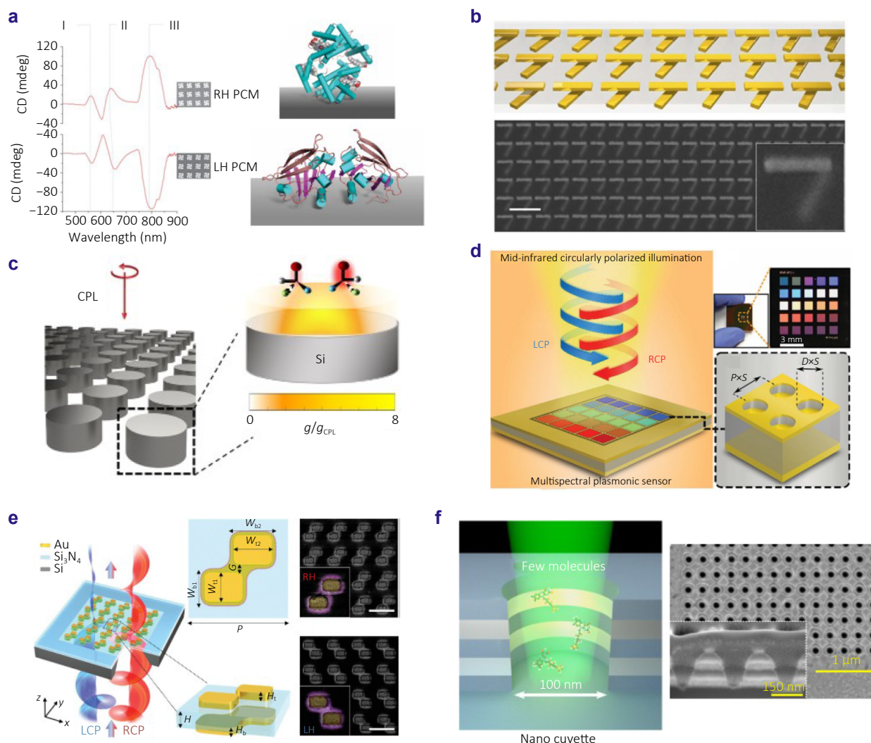
Fig. 13 | Metasurface-enhanced chiral sensing strategies. (a) Planar chiral metamaterials generating superchiral near fields for ultrasensitive biomolecular detection. (b) Twisted plasmonic metamaterials allowing zeptomole detection. (c) Dielectric metasurfaces leveraging Mie resonances for large-volume, low-loss chiral sensing. (d) Pixelated IR metasurfaces enabling vibrational chiral barcoding of molecular mixtures. (e–f) Suspended metasurfaces 253 and negative-index nanocavities achieving ultrathin and highly sensitive enantiodiscrimination. Figure reproduced with permission from: (a) ref. 48 , Springer Nature; (b) ref. 234 , under a Creative Commons CC BY license; (c) ref. 53 , American Chemical Society; (d) ref. 239 , Wiley-VCH GmbH; (e) ref. 253 , Wiley-VCH GmbH; (f) ref. 240 , American Chemical Society.
