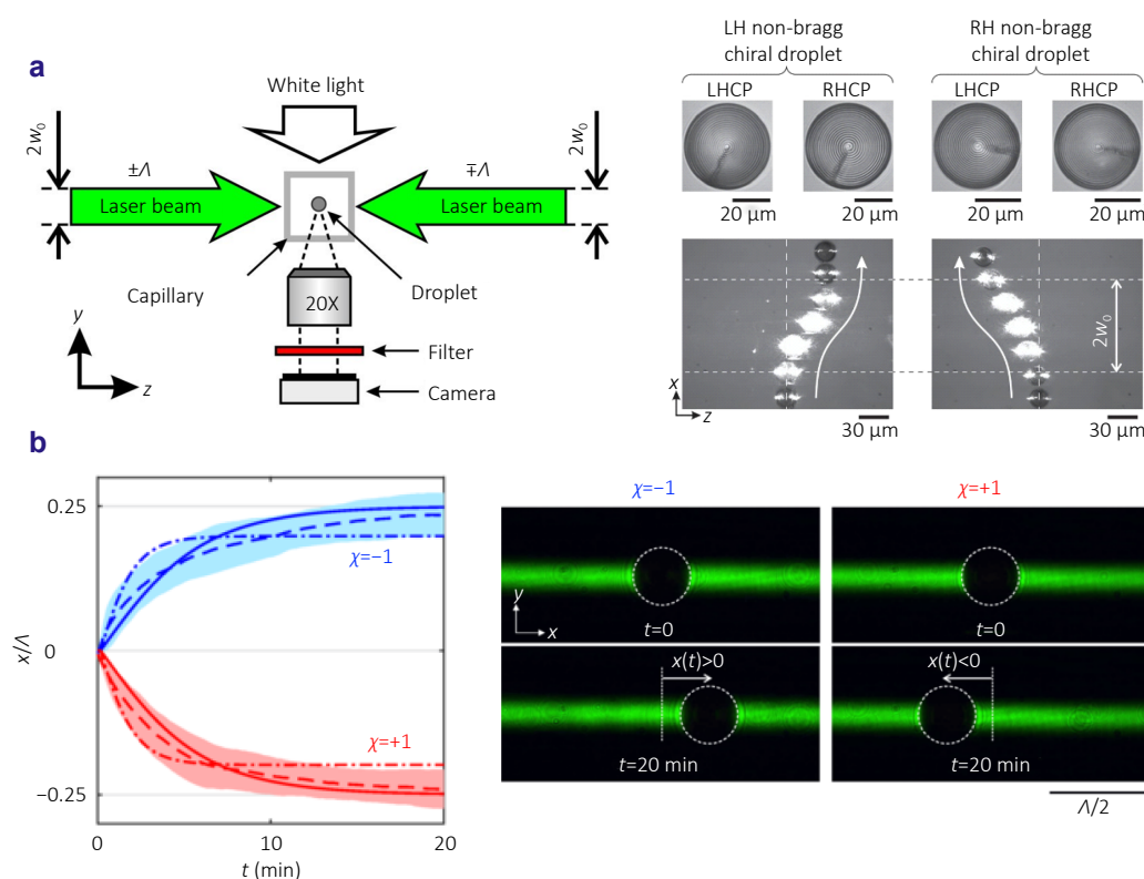
Fig. 5 | Optical radiation pressures and optical gradient forces for chiral sorting. (a) ORP using counter-propagating beams of opposite helicity, enabling opposite enantiomers to move in opposite directions. (b) Helicity-dependent displacement of particles arising from OGF, which is strongly correlated with the chiral polarizability of the analytes. Figure reproduced with permission from: (a) ref. 110 , Springer Nature; (b) ref. 39 , American Physical Society.
