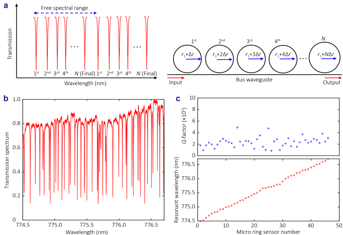
Fig. 2 | (a) Schematic diagram of the proposed micro-ring resonator array. (b) Measured transmittance of 50 elements of micro-ring array. (c) Quality factor of each ring (top) and sequence information (bottom).
