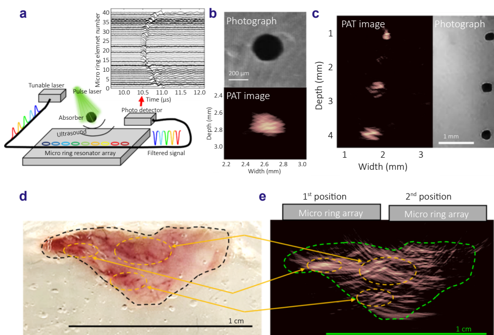
Fig. 4 | (a) Experimental configuration of PAT of a single black sphere. The inset figure shows the measured photoacoustic signals of the black sphere captured by the 40 elements of the micro-ring array. (b) Reconstructed image (bottom) from the acquired PAT signals and photograph (top) of the black sphere. (c) Photograph of multiple black spheres (right) and the reconstructed PAT image acquired by the micro-ring array (left). (d) Photograph of half of a mouse prostate and (e) the reconstructed PAT image of the prostate tissue acquired by the micro-ring array.
