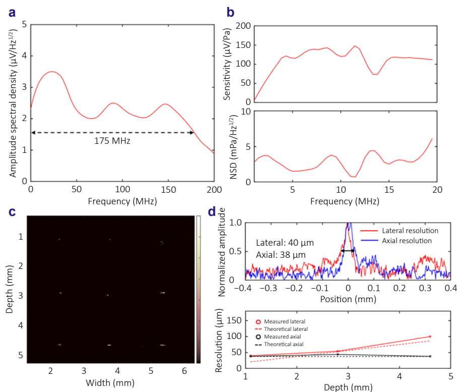
Fig. 5 | (a) Measured amplitude spectral density of a micro-ring using a broadband acoustic source. (b) Measured receiving sensitivity of the micro-ring (top) and NEP spectral density (bottom) using a calibrated hydrophone and a 10 MHz transducer. (c) Combined PAT image showing the acoustic point source placed at 3 by 3 different spot locations. (d) Measured lateral and axial resolution at the 1.1 mm depth along the center of the micro-ring array (top), and the measured lateral and axial resolutions at different depths along the center vs. the theoretical values (bottom).
