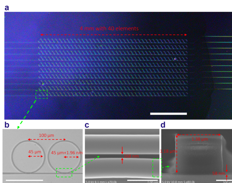
Fig. 3 | Photographs and SEM images of fabricated micro-ring resonator arrays using NIL method. (a) Photograph of micro-ring arrays under microscope with several lines with different gap sizes between the micro-rings and the bus waveguides (1 mm scale bar). (b) Photograph of two micro-ring resonators and a bus waveguide (100 \mu\text{m} scale bar). (c) SEM images of the gap between the bus waveguide and the micro-ring and (d) the cross section of the bus waveguide.
