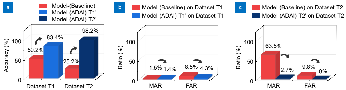
Fig. 8 | (a) The accuracies of Model-(Baseline), Model-(ADAI)-T1', and Model-(ADAI)-T2' on Dataset- T1 and Dataset-T2. The MAR and FAR of (b) Model-(Baseline) and Model-(ADAI)-T1' on Dataset-T1, and (c) Model-(Baseline) and Model-(ADAI)-T2' on Dataset-T2, respectively.
