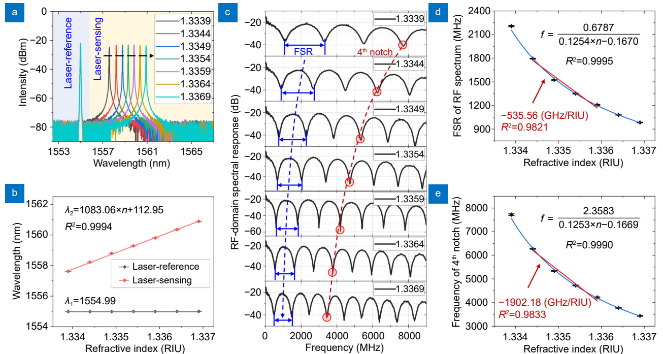
Fig. 4 | (a) Dual-wavelength laser spectra in solutions with different RIs. (b) Fitting relationship between laser wavelength and RI. (c) RF spectrum in solutions with different RIs. (d) FSR response with RI and its fitting curve. (e) The 4th notch frequency response with RI and its fitting curve.
