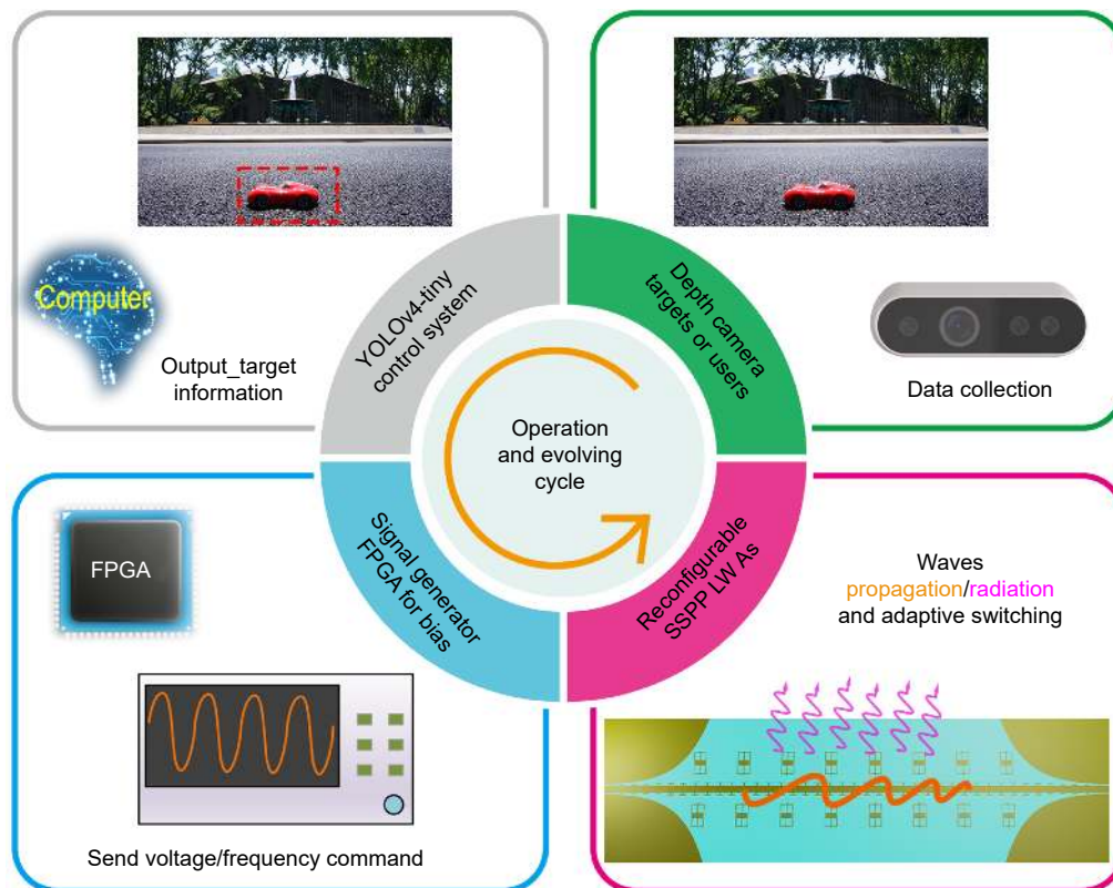
Fig. 2 | Smart SSPP-LWA operation architecture. There are four main components in the operation cycle. The depth camera is used for capturing picture information. Through the control system based on YOLOv4-tiny pre-training module, the target detection task is completed. Two devices, the FPGA and the signal generator, are used to control the voltage and input frequency signal to control the reconfigurable SSPP-LWA. Finally, the smart SSPP-LWA can realize the adaptive real-time switching between the radiation and the non-radiation of EM waves and beam tracking.
