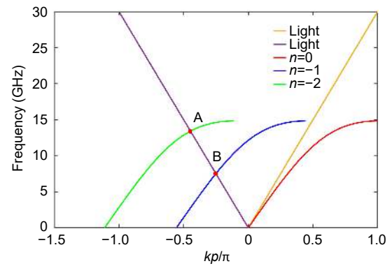
Fig. 3 | Dispersion curves of space harmonics.
