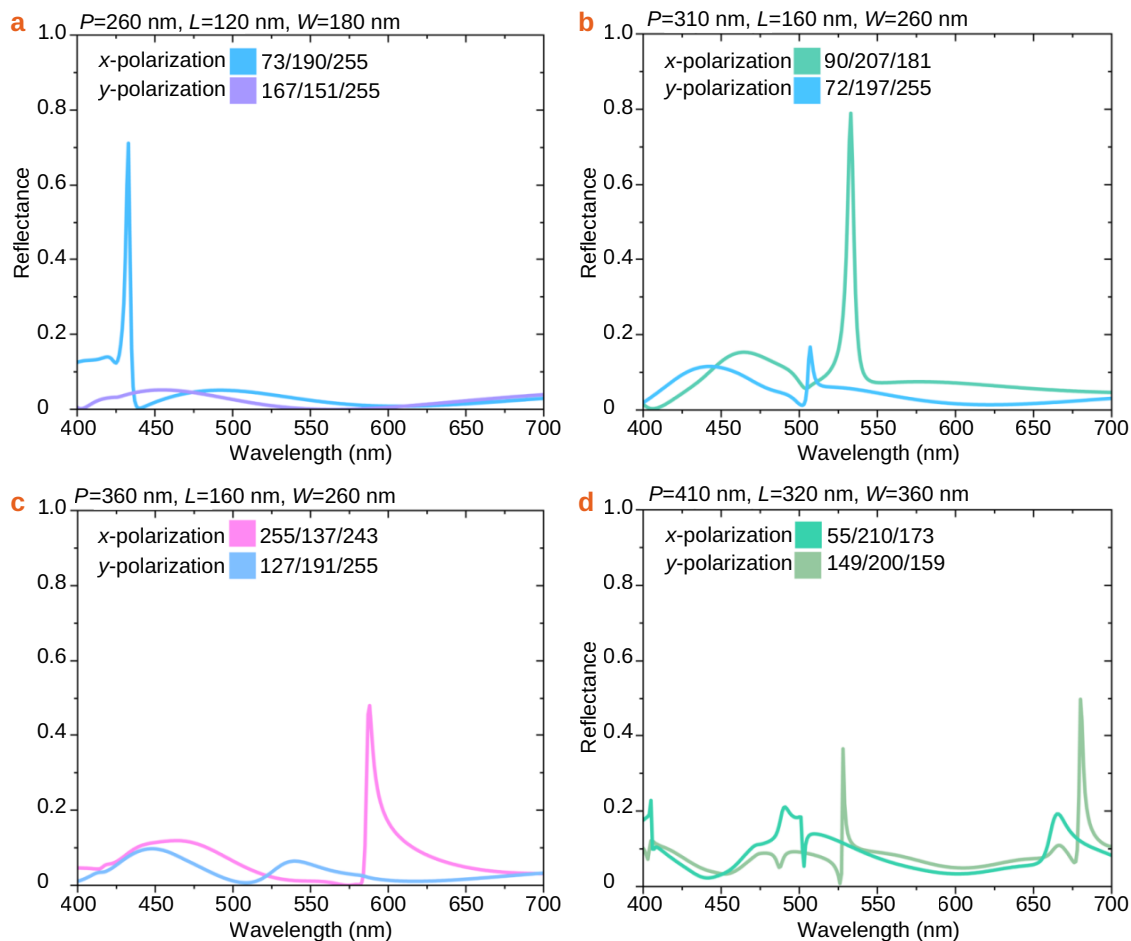
Fig. 2 | (a)–(d) Comparison of reflection spectra for several sets of nanostructural parameters under normal incidence with x - and y -polarized illumination. The structural colors are visualized based on the calculated reflection spectra, with the luminance component ( Y ) uniformly normalized to 0.5.
