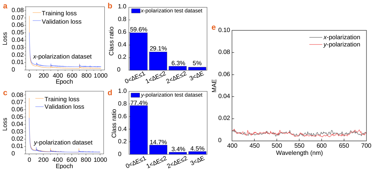
Fig. 4 | (a) and (c) Training and validation losses under x-polarization and y-polarization. (b) and (d) Statistical distributions of the color difference between predicted and target colors for x-polarization and y-polarization directions. (e) Distribution of spectral prediction errors under different polarization conditions.
