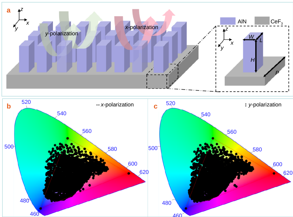
Fig. 1 | (a) Schematic of the investigated polarization-selective metasurface based on AlN nanostructures, along with the geometric parameters, including the nanocolumn length ( L ), width ( W ), height ( H ), and period ( P ). (b)–(c) Colors of the training dataset as displayed on the CIE 1931 color space chromaticity diagram, (b) x -polarization direction, and (c) y -polarization direction.
