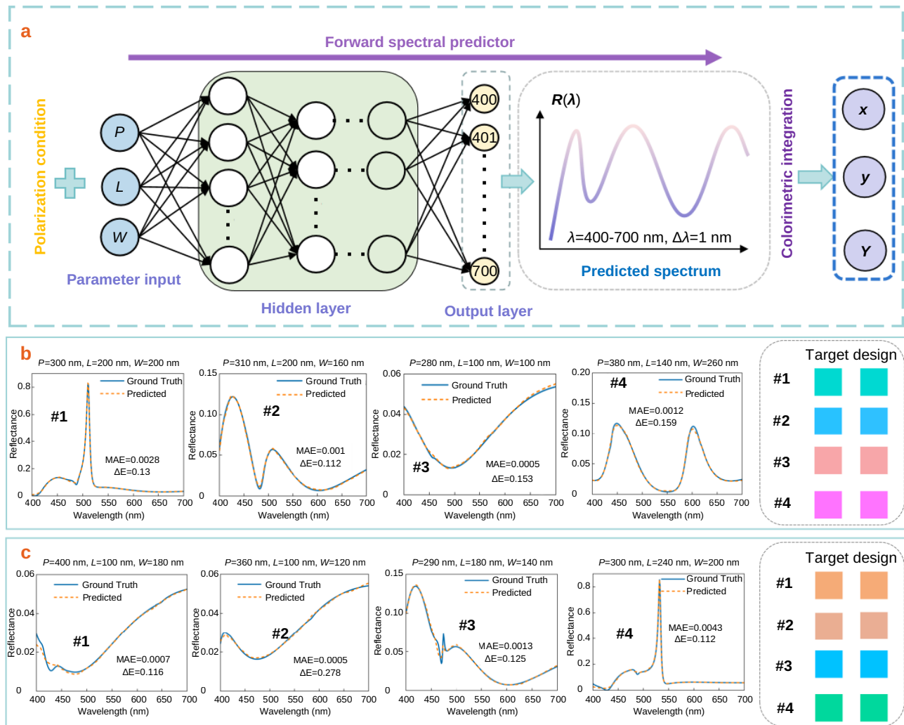
Fig. 3 | (a) Schematic diagram of the model structure, with structural parameters as inputs under different polarization conditions, and reflection spectra in the 400–700 nm range as outputs, which are further converted to a color space. (b) Spectral prediction results for a typical sample under x-polarization; the blue line represents the actual values, and the orange line represents the predicted values. (c) Spectral prediction results for a typical sample under y-polarization; the blue line represents the actual values, and the orange line represents the predicted values.
