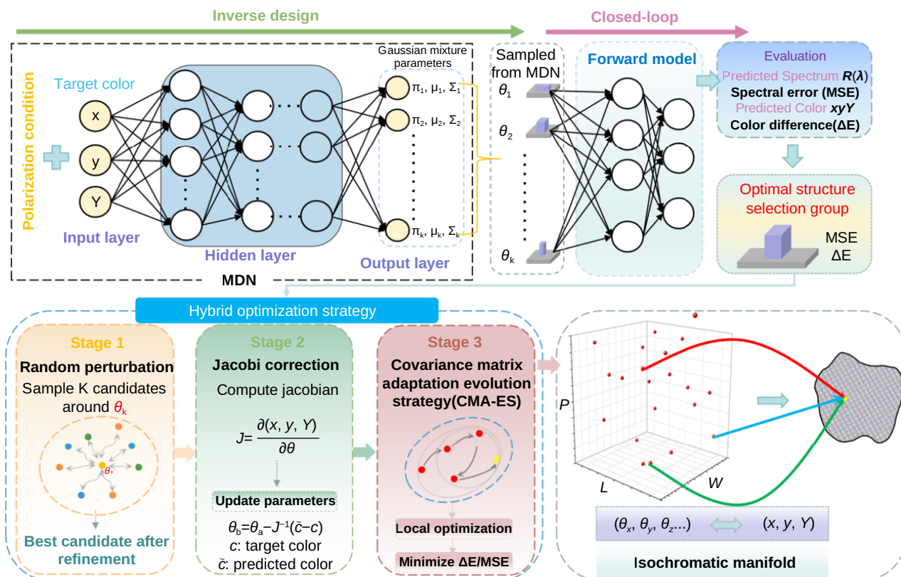
Fig. 5 | Schematic diagram of a framework for the inverse design of structural color based on a mixture density network and a hybrid optimization strategy.
