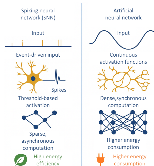
Fig. 2 | Difference and advantages of SNN compared to ANN.
