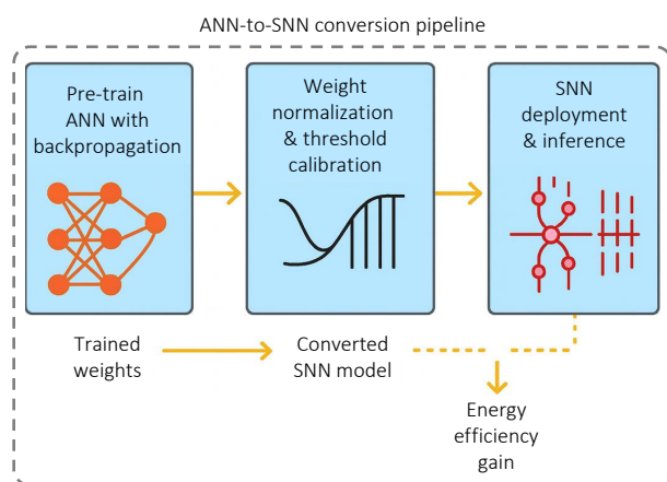
Fig. 4 | Generic ANN-to-SNN conversion pipeline. This diagram illustrates the transformation process, highlighting how a pre-trained ANN is adapted to an SNN, typically involving threshold mapping and weight transfer to leverage existing deep learning successes.
